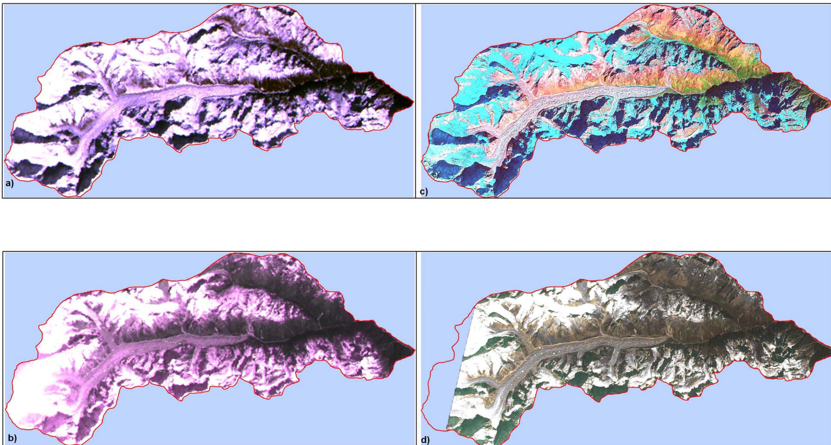
Fig. 3.12 Satellite Images showing the Zemu glaciers with different dates: a) November, 1989 Landsat-4 TM; b) November, 1990 IRS-1C LISS-II; c) December, 2000 Landsat ETM+ and d) November, 2002 IRS-1D LISS-III
