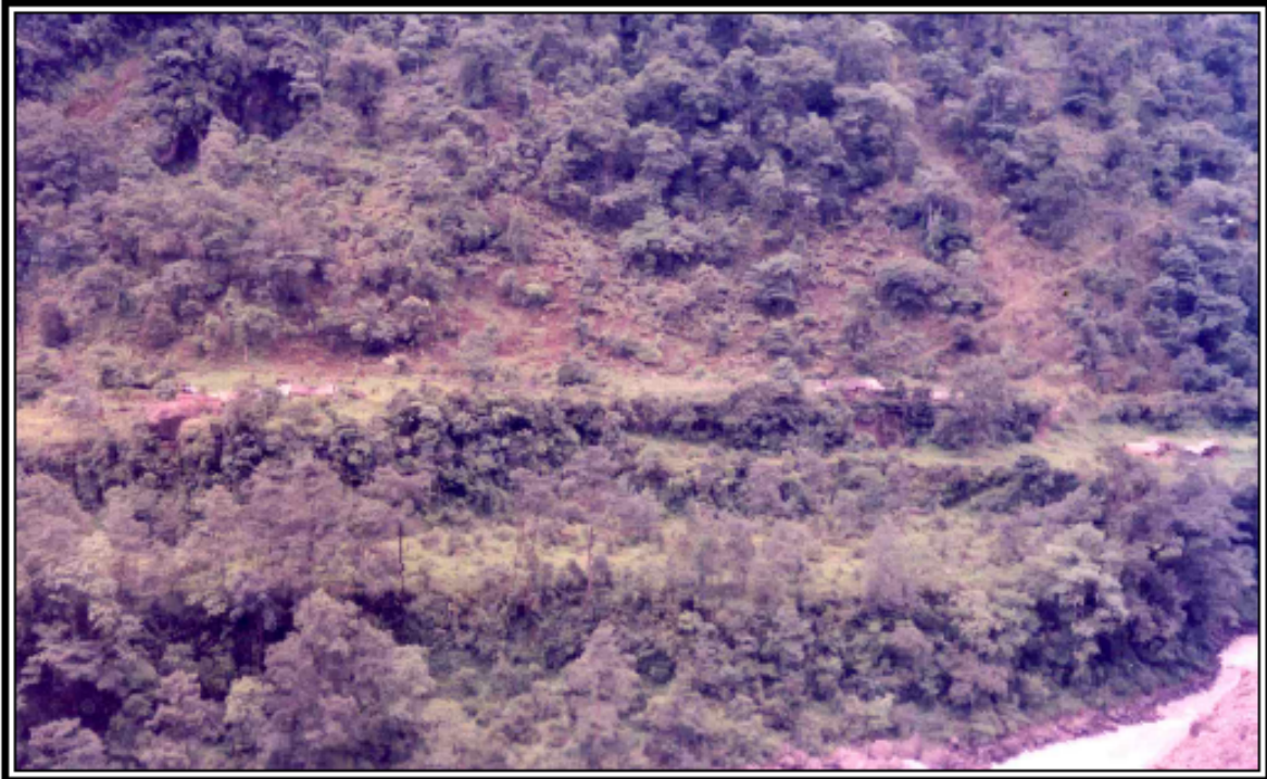
Plate 1.1 River terraces at the confluence of Teesta river and Chakung Chhu
