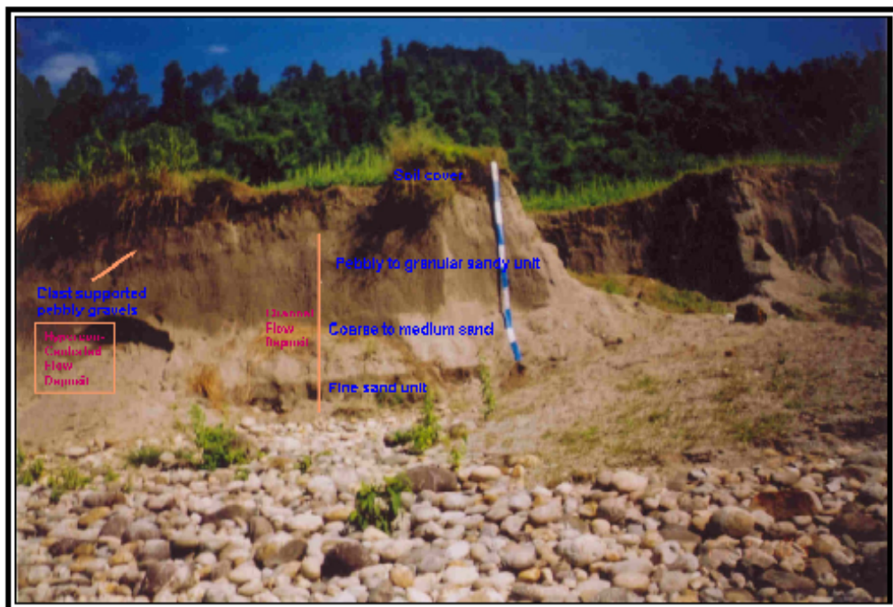
Plate 1.7c Terrace near Ralap village with hyperconcentrated and stream flow deposits
