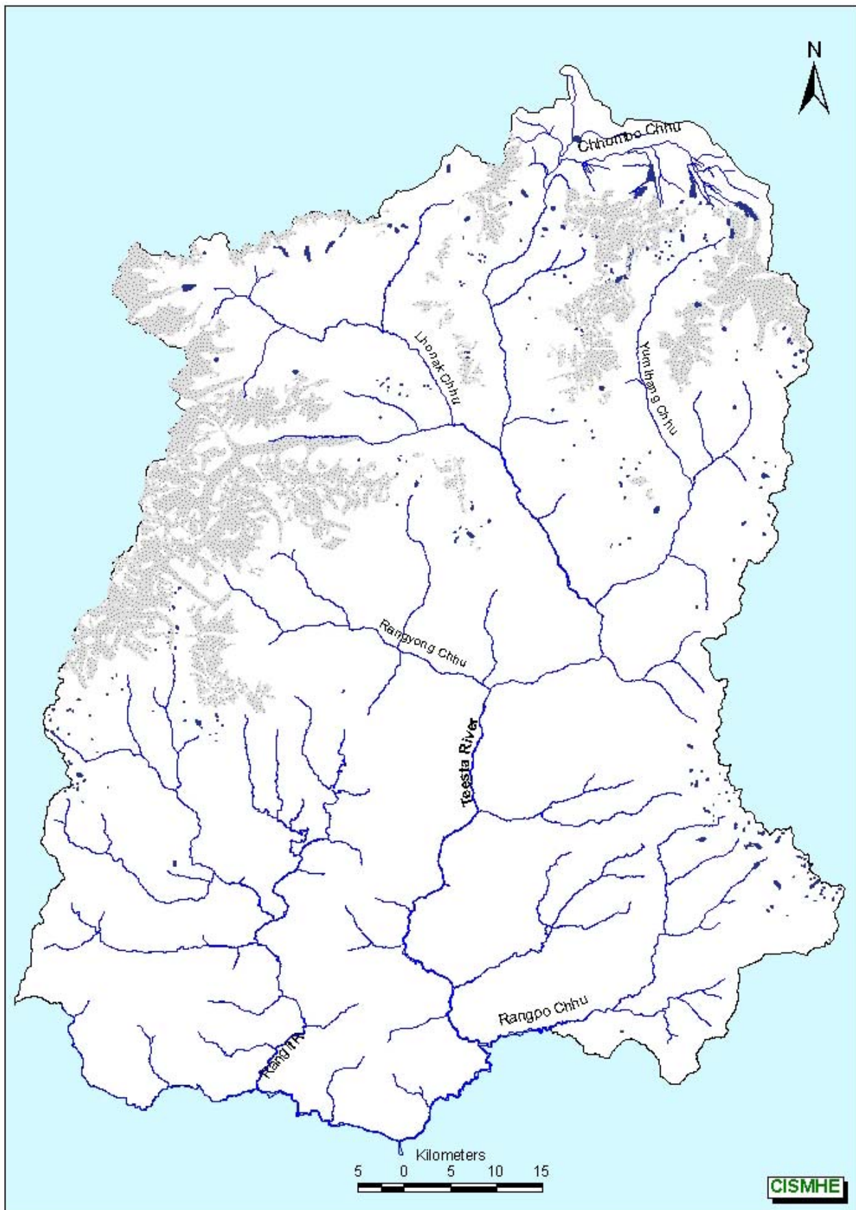
Fig.10 Glaciers and lakes of Sikkim Himalaya
