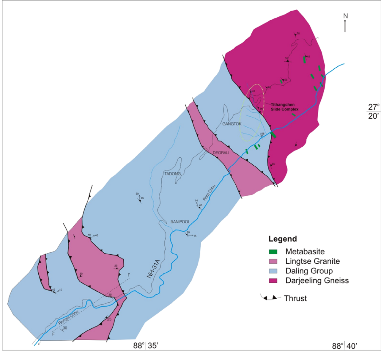
Fig.2.6 Geology of the area around Gangtok with locations of Chandmari-Tithangchen slide complex and 9 th mile slide.
