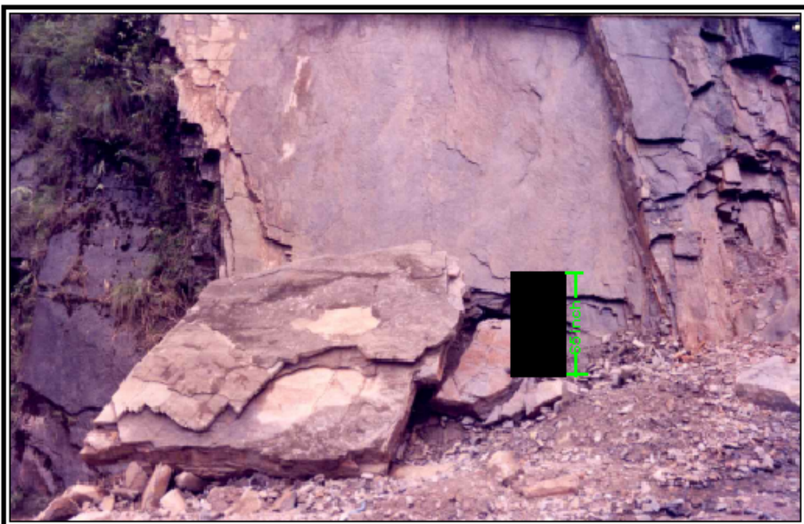
Plate 1.4 Rhombohedral blocks separated out from the rock mass by plane failure mode
