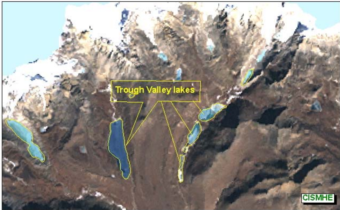
Fig. 3.17 Trough valley lakes formed along the river valley in North Sikkim
