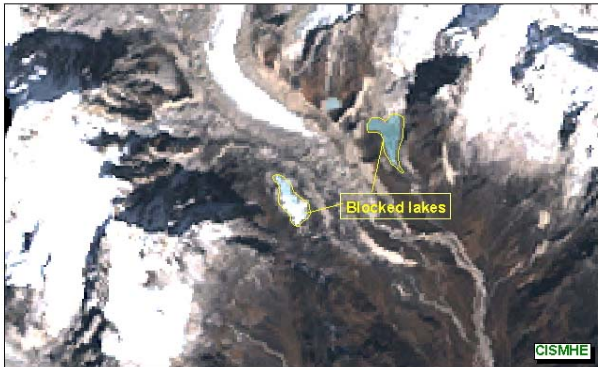
Fig. 3.18 The blocked lakes formed adjacent to the glacier by blocking in North Sikkim
